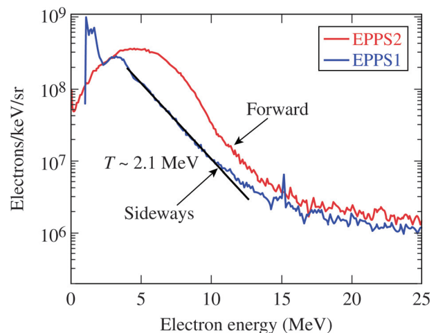
FIG. 9. (Color online) Fast-electron spectra measured in the laser's forward direction and perpendicular to the laser direction (Shot 59124).
