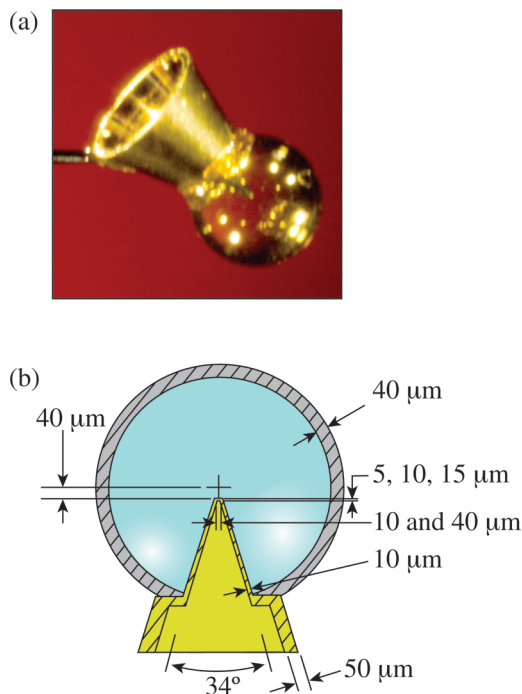
FIG. 2. (Color online) (a) Photograph of a gold re-entrant cone target; (b) cross-sectional drawing through the shell and cone tip with target dimensions.
