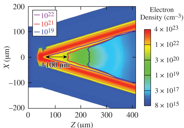
FIG. 11. (Color online) Electron-density contours from a 2D HYDRA simulation at the time of the short-pulse interaction of the preplasma formation in a gold cone with inner tip diameter of 10\ \mu\text{m} .
