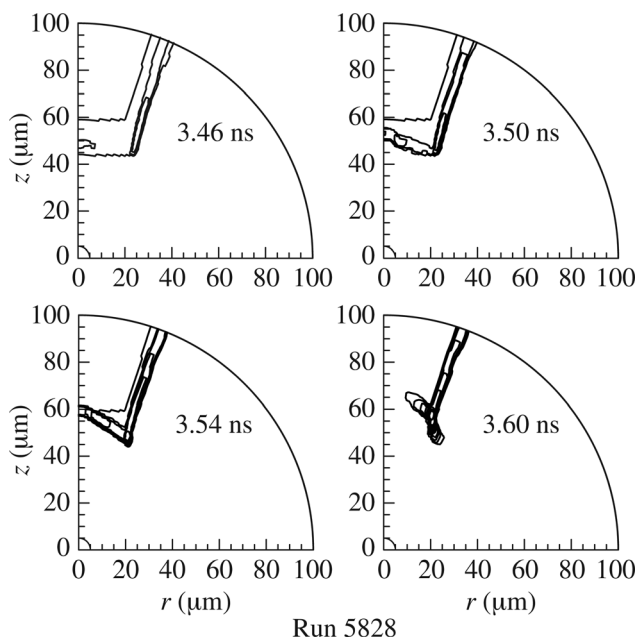
FIG. 5. Sequence of density contours above 10 \text{ g/cm}^3 in the tip of an Au cone from a 2D SAGE simulation, showing the rapid propagation of a strong shock wave through a 15- \mu\text{m} cone tip. The fuel assembly from a cone-in-shell target (not shown) generates the shock. The shock propagates faster through the cone tip than through the wall.
