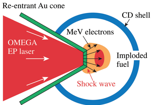
FIG. 1. (Color online) Schematic of the integrated cone-in-shell fast-ignition experiment.
