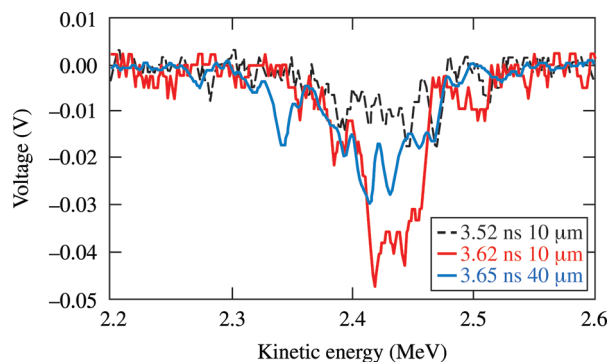
FIG. 7. (Color online) Time-of-flight spectra of 2.45 MeV neutrons from thermonuclear d(d,n)^3\text{He} reactions in integrated fast-ignition experiments. Spectra with various timings of the OMEGA EP beam are shown for two target types.
