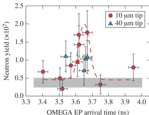
FIG. 8. (Color online) Measured neutron yield as a function of the arrival time of the short-pulse laser for 10- \mu\text{m} (circles) and 40- \mu\text{m} (triangles) tip diameter cone targets. The gray area represents data without the short-pulse laser.
