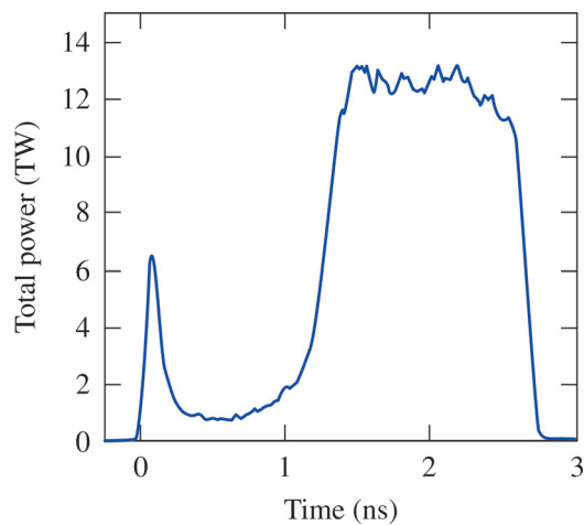
FIG. 3. (Color online) Drive laser pulse shape (Shot 55154).
