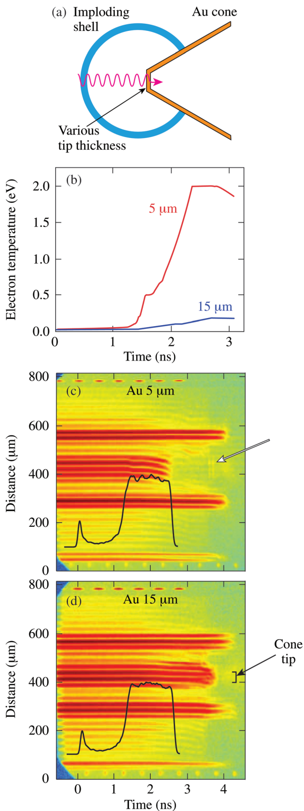
FIG. 6. (Color online) (a) Schematic for simulations of radiation preheat of the cone tip. Coronal x-ray radiation from the shell driven by the strong UV pulse can penetrate through the cone wall, preheating the gold material. (b) Calculated electron temperature at the inside of the cone tip for 5 and 15 \mu\text{m} thicknesses. (c) VISAR trace for a 5 \mu\text{m} thickness, the disappearance of the fringes at \sim 2.5 ns indicate preheat. The white arrow marks the optical emission at the shock-breakout time. (d) VISAR trace for a 15 \mu\text{m} thickness, showing no attenuation before shock breakout at 3.75 ns. The brace indicates the spatial range of the flat tip. In (c) and (d) the black curve indicates the laser's temporal shape.
