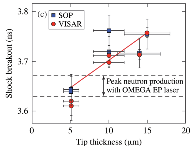
FIG. 4. (Color online) (a) Schematic of the shock-breakout experiment. The CD shell was imploded using just the long-pulse, 351-nm drive beams, resulting in shock propagation through the tip of the cone. Emergence of the shock at the inside of the tip was diagnosed using an SOP and VISAR, (b) SOP trace for a typical shot, and (c) measured breakout time inside the cone for various tip thicknesses. The breakout is later for thicker cone tips.
