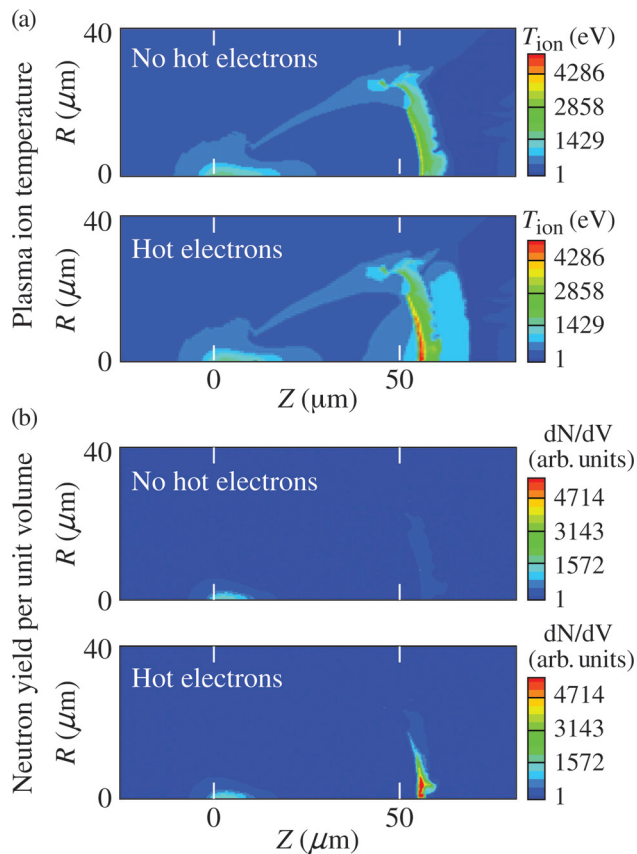
FIG. 10. (Color online) DRACO + LSP simulation for a 10-ps, 1.0-kJ, R_{80} = 27\text{-}\mu\text{m} OMEGA EP pulse, showing contours of (a) plasma ion temperature and (b) neutron yield per unit volume, with and without hot electrons produced by the OMEGA EP pulse.
